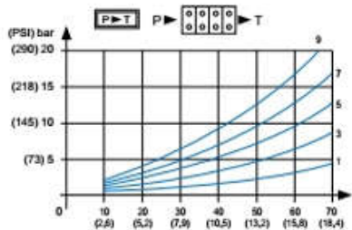
Characteristic Pressure Drop
